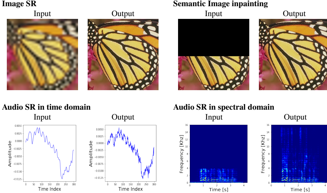
Fig. 2. Illustration of the input output for image SR, semantic image inpainting, and audio SR in time and frequency domain. Audio SR in time domain is analogous to image SR, where “edges” are missing in the LR input. On the other hand, Audio SR in spectral domain can be viewed as image inpainting of spectrograms, i.e. , given the bottom low frequency “image”, predict the remaining image.
