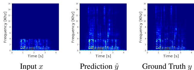
Fig. 1. Spectrogram corresponding to the LR input (frequencies above 4kHz missing), HR reconstruction, and the HR ground truth. Our approach successfully recovers the high frequency components from the LR audio signal.
